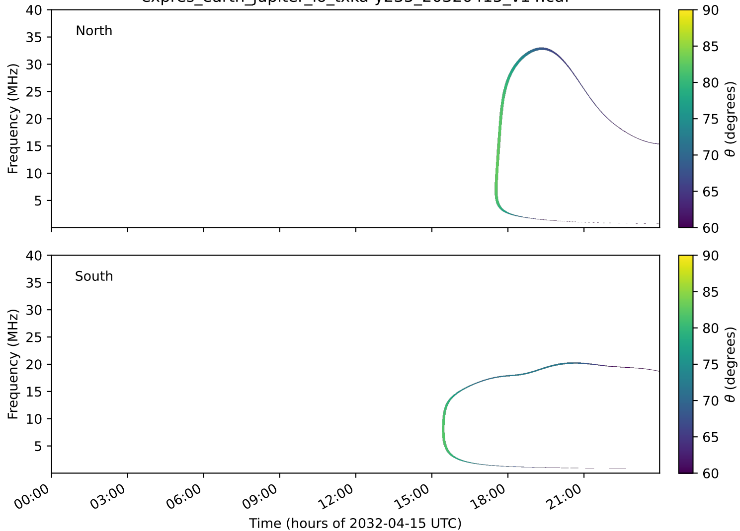
expres_earth_jupiter_io_txka-y235_20320415_v14.cdf
