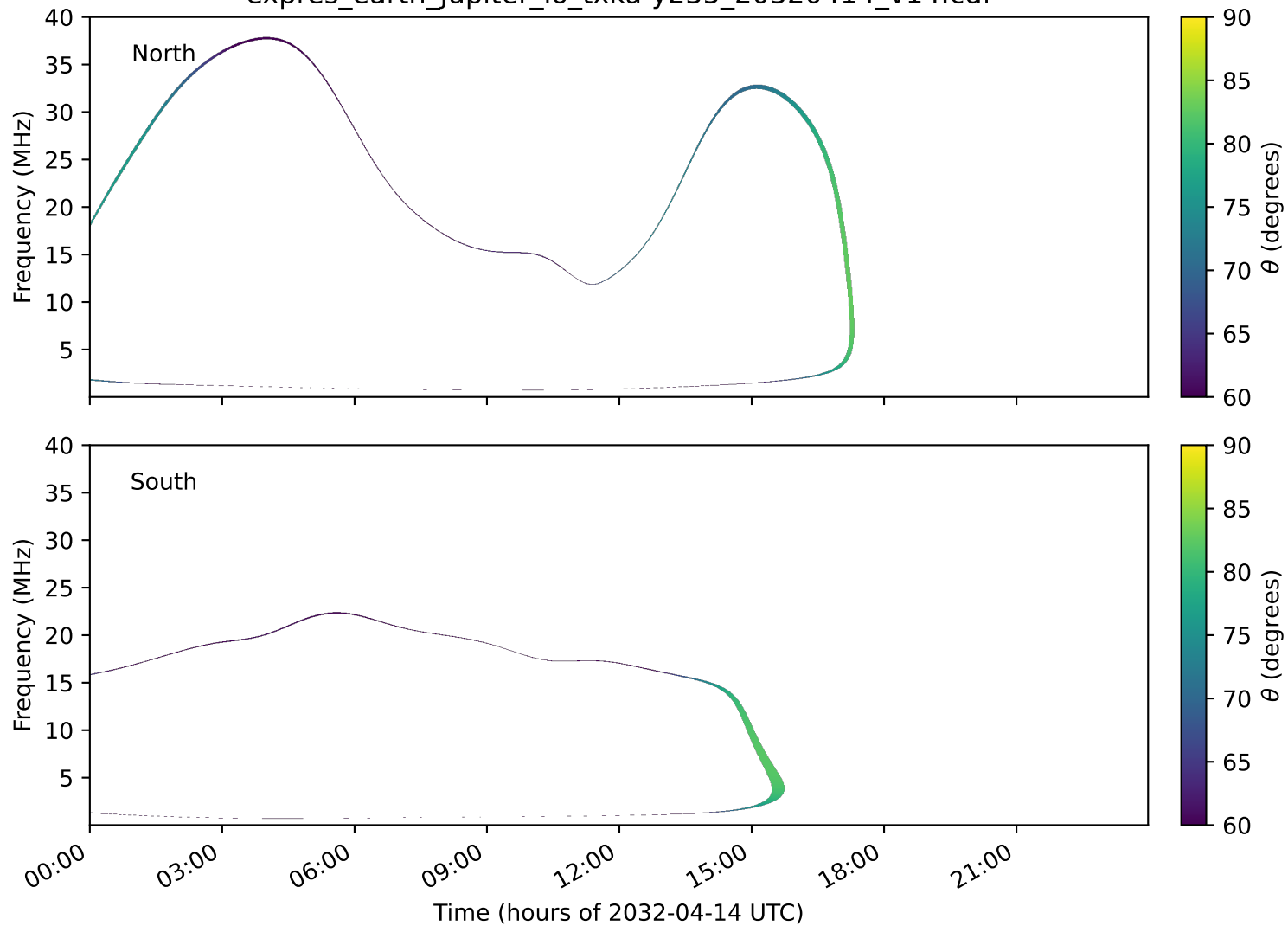
expres_earth_jupiter_io_txka-y235_20320414_v14.cdf
