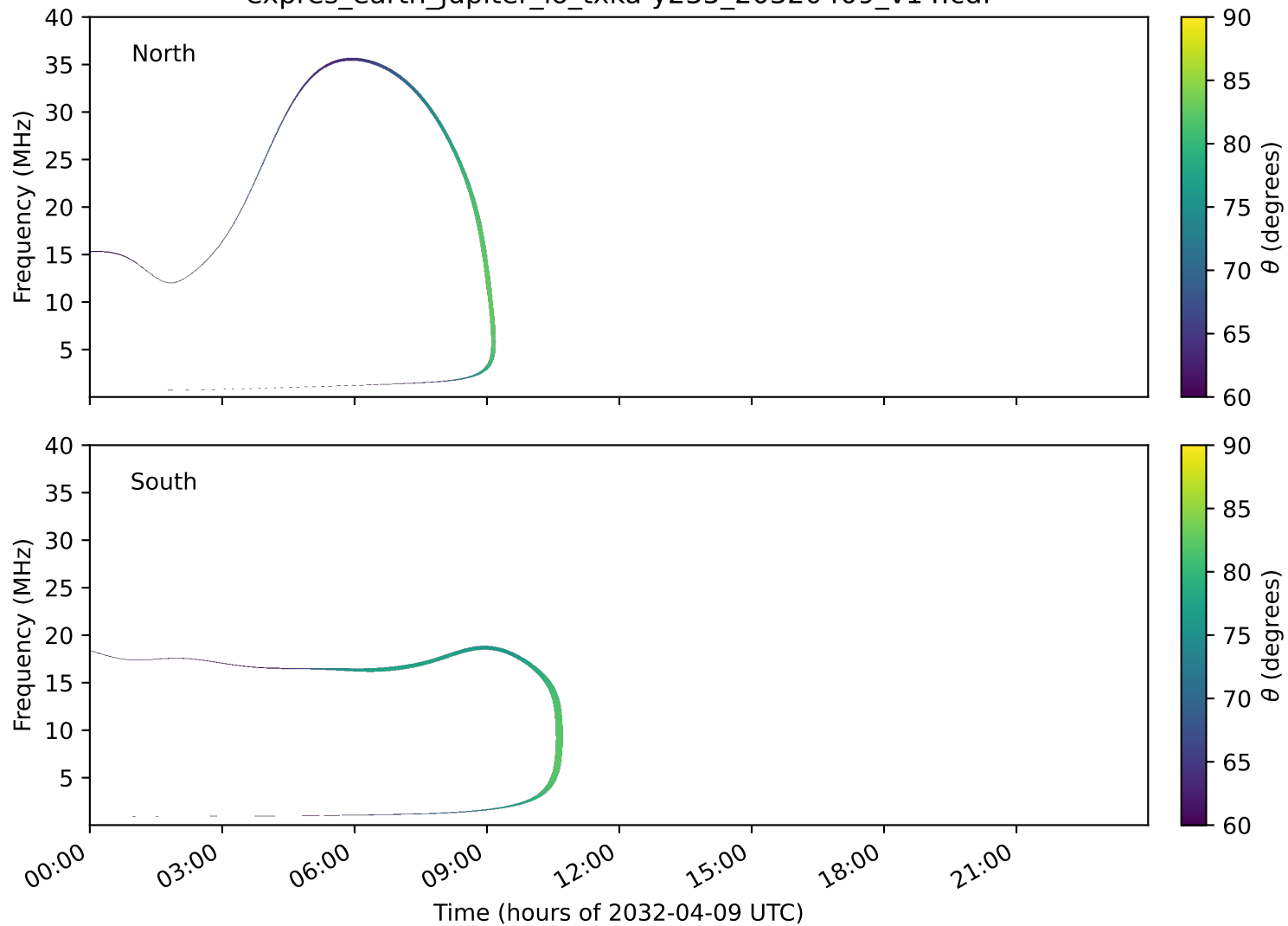
expres_earth_jupiter_io_txka-y235_20320409_v14.cdf
