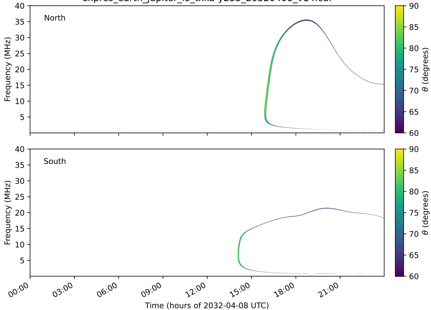
expres_earth_jupiter_io_txka-y235_20320408_v14.cdf
