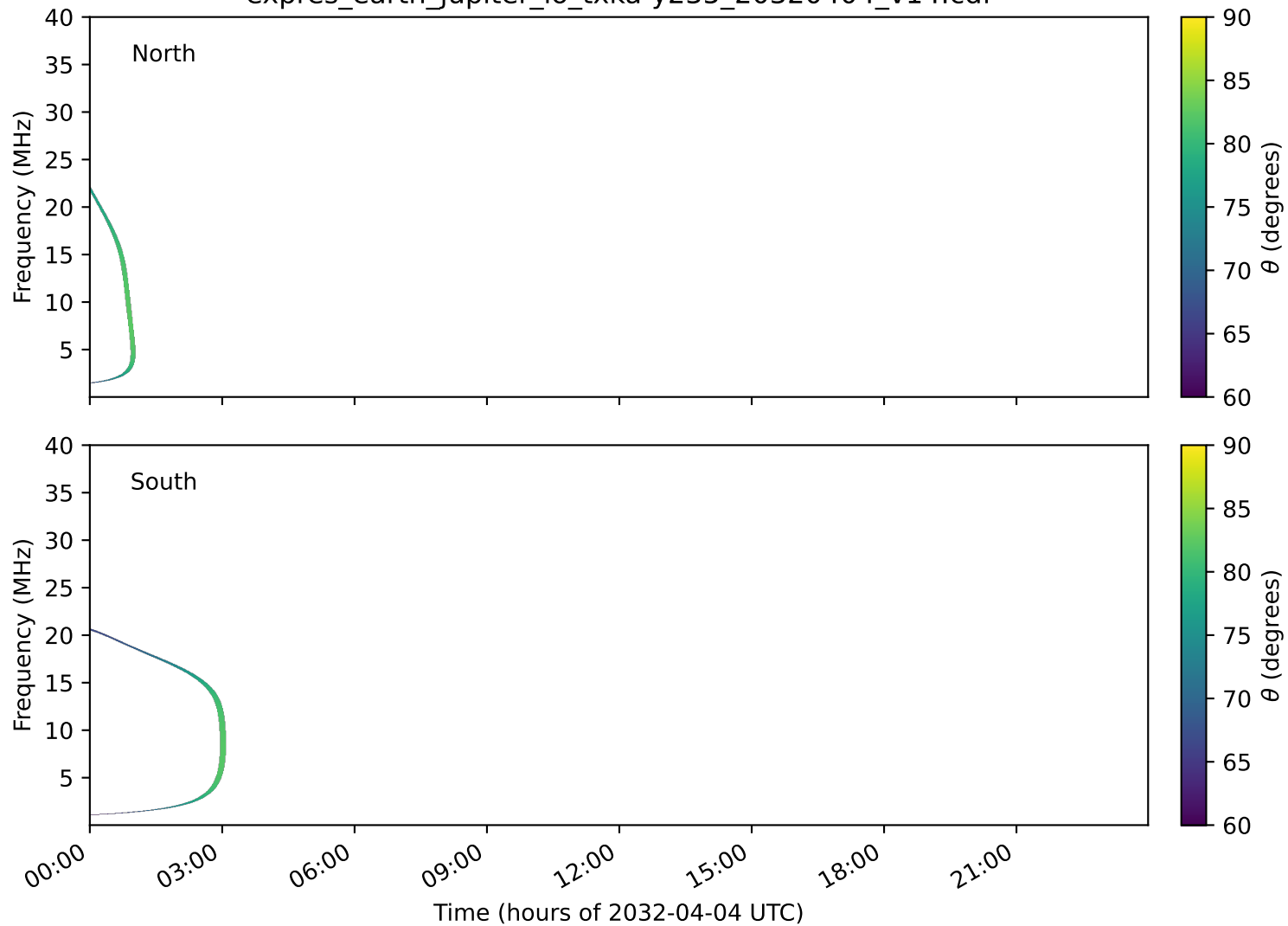
expres_earth_jupiter_io_txka-y235_20320404_v14.cdf
