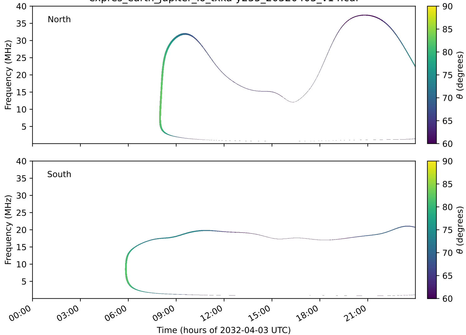
expres_earth_jupiter_io_txka-y235_20320403_v14.cdf
