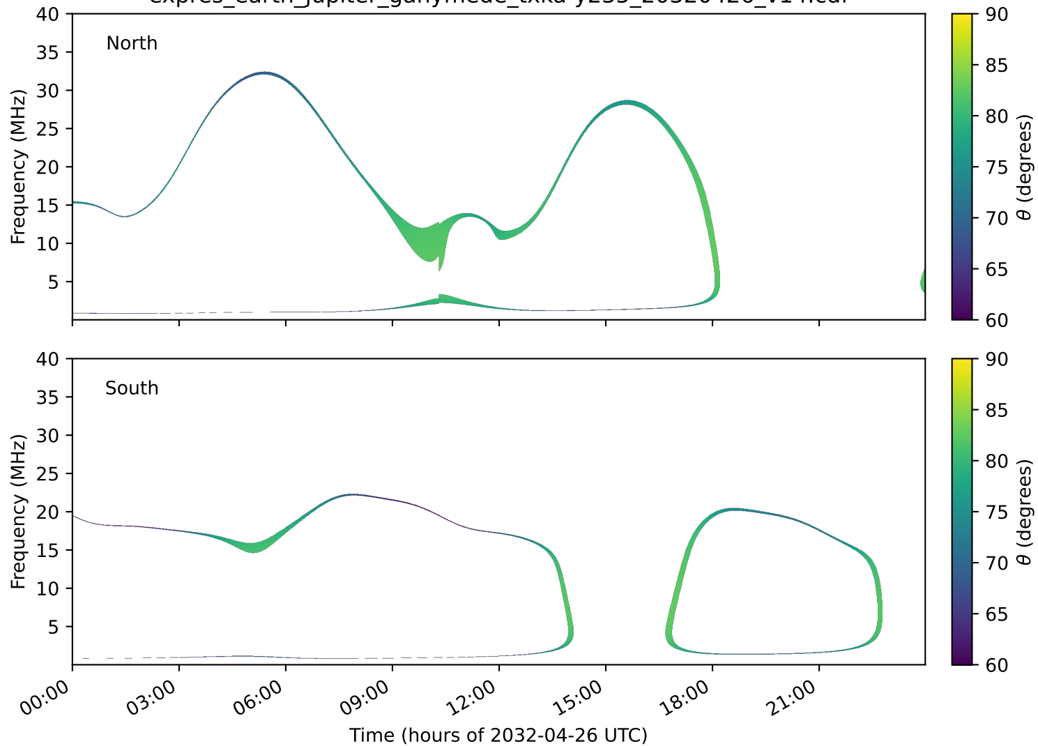
expres_earth_jupiter_ganymede_txka-y235_20320426_v14.cdf
