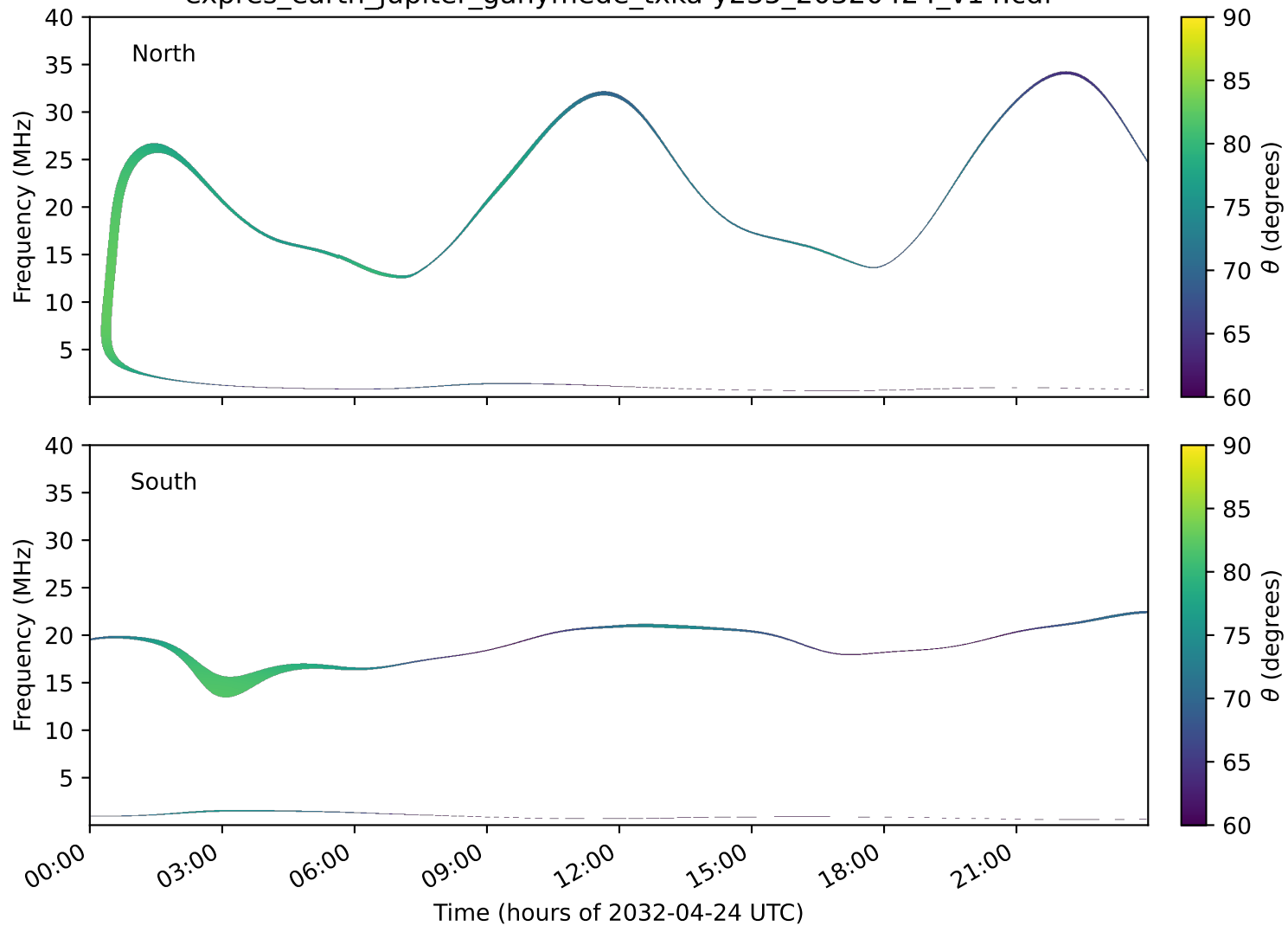
expres_earth_jupiter_ganymede_txka-y235_20320424_v14.cdf
