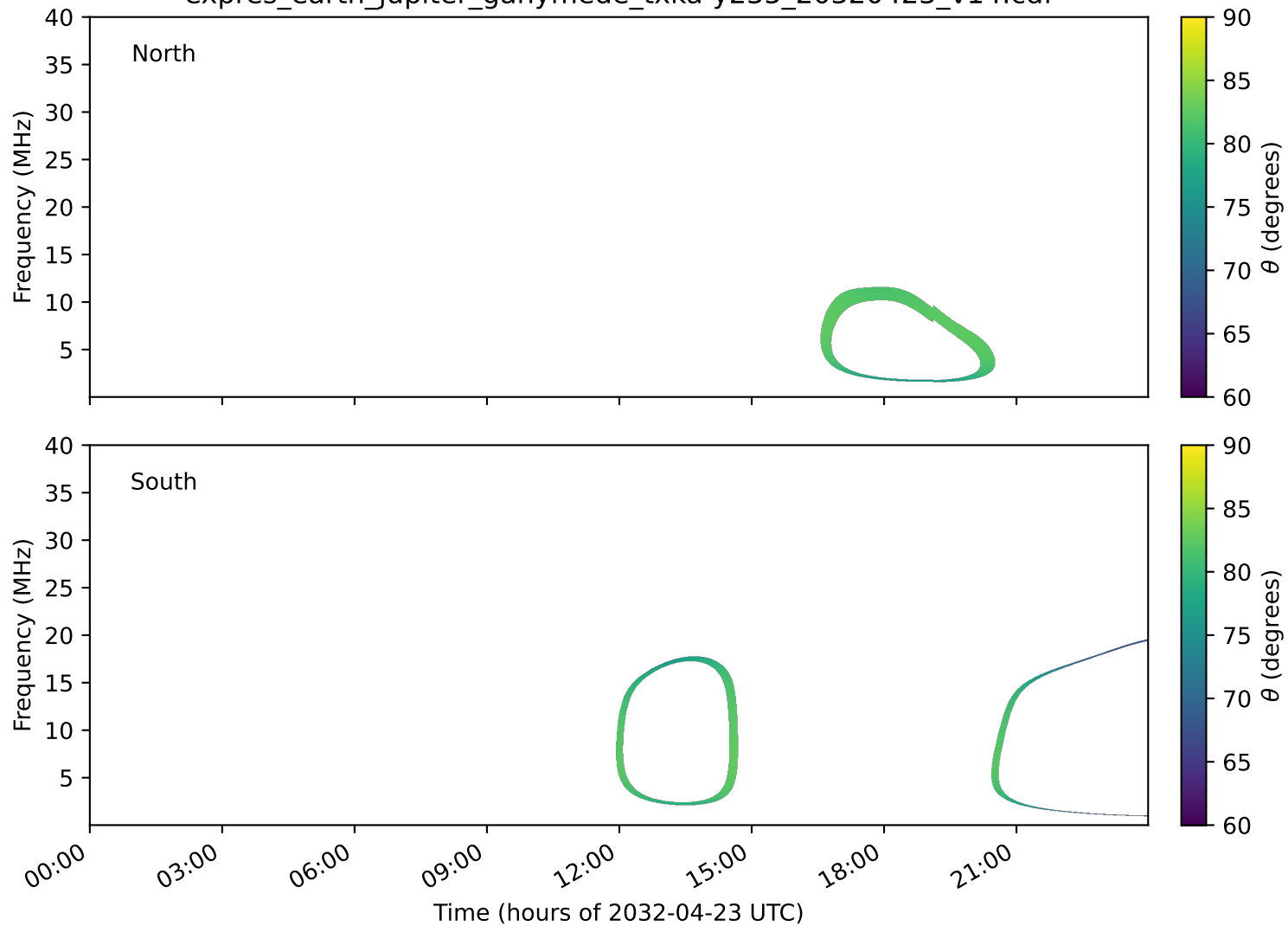
expres_earth_jupiter_ganymede_txka-y235_20320423_v14.cdf
