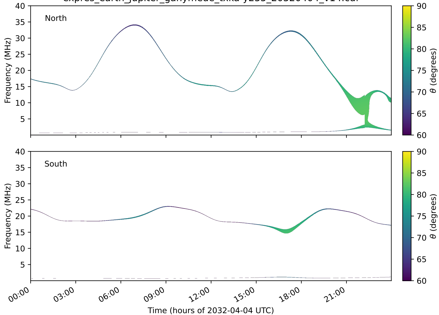
expres_earth_jupiter_ganymede_txka-y235_20320404_v14.cdf
