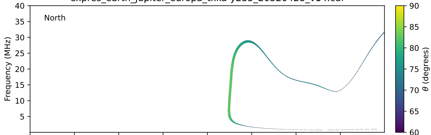
expres_earth_jupiter_europa_txka-y235_20320428_v14.cdf
