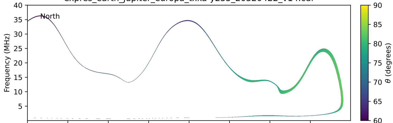
expres_earth_jupiter_europa_txka-y235_20320422_v14.cdf
