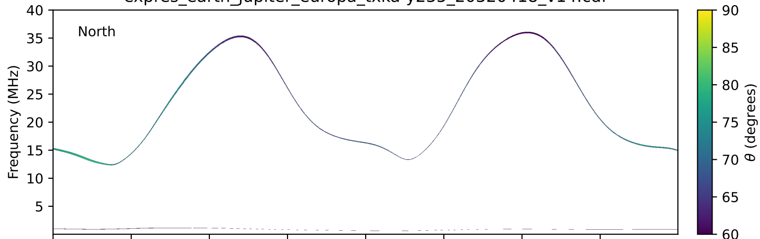
expres_earth_jupiter_europa_txka-y235_20320418_v14.cdf
