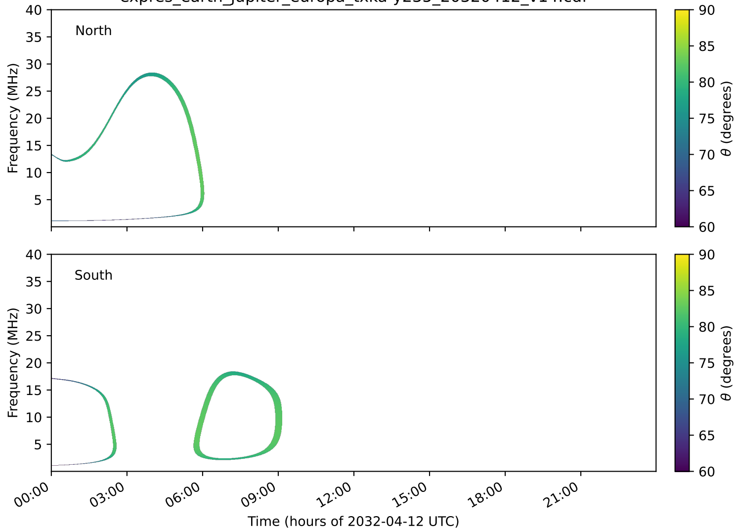
expres_earth_jupiter_europa_txka-y235_20320412_v14.cdf
