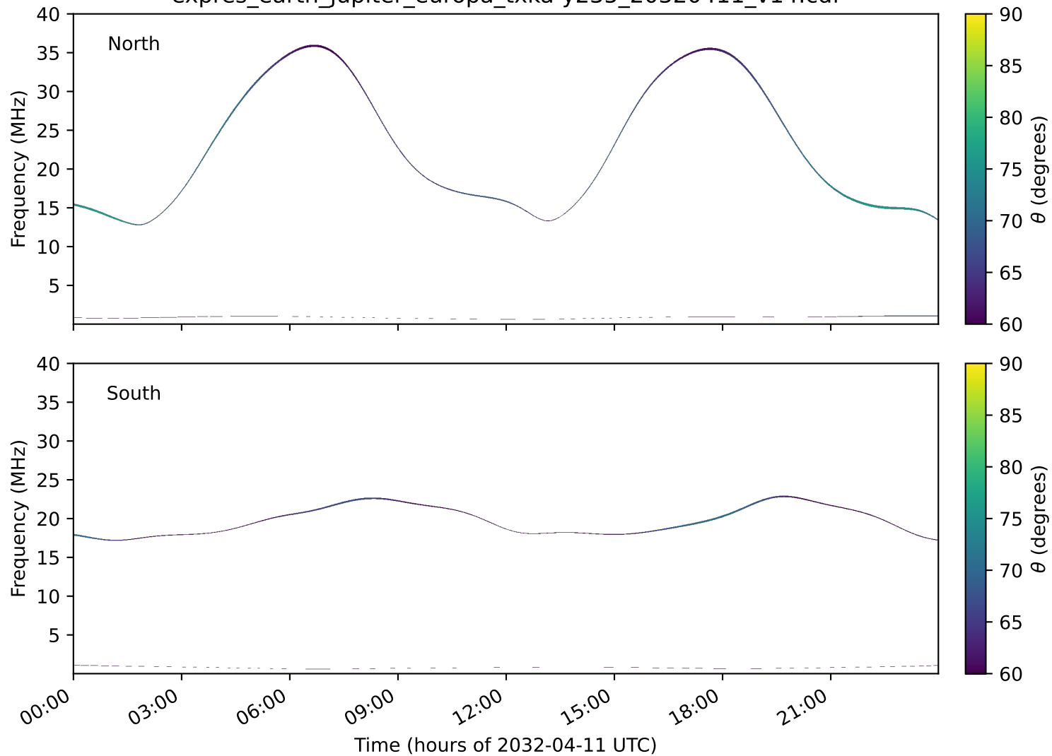
expres_earth_jupiter_europa_txka-y235_20320411_v14.cdf
