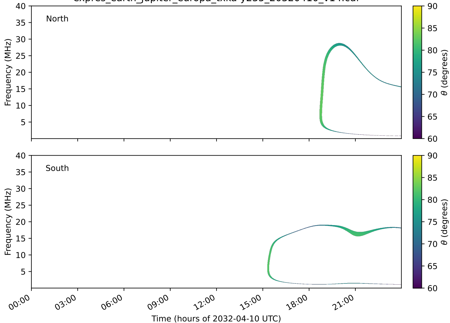
expres_earth_jupiter_europa_txka-y235_20320410_v14.cdf
