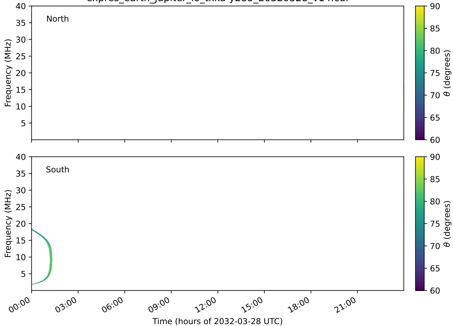
expres_earth_jupiter_io_txka-y235_20320328_v14.cdf
