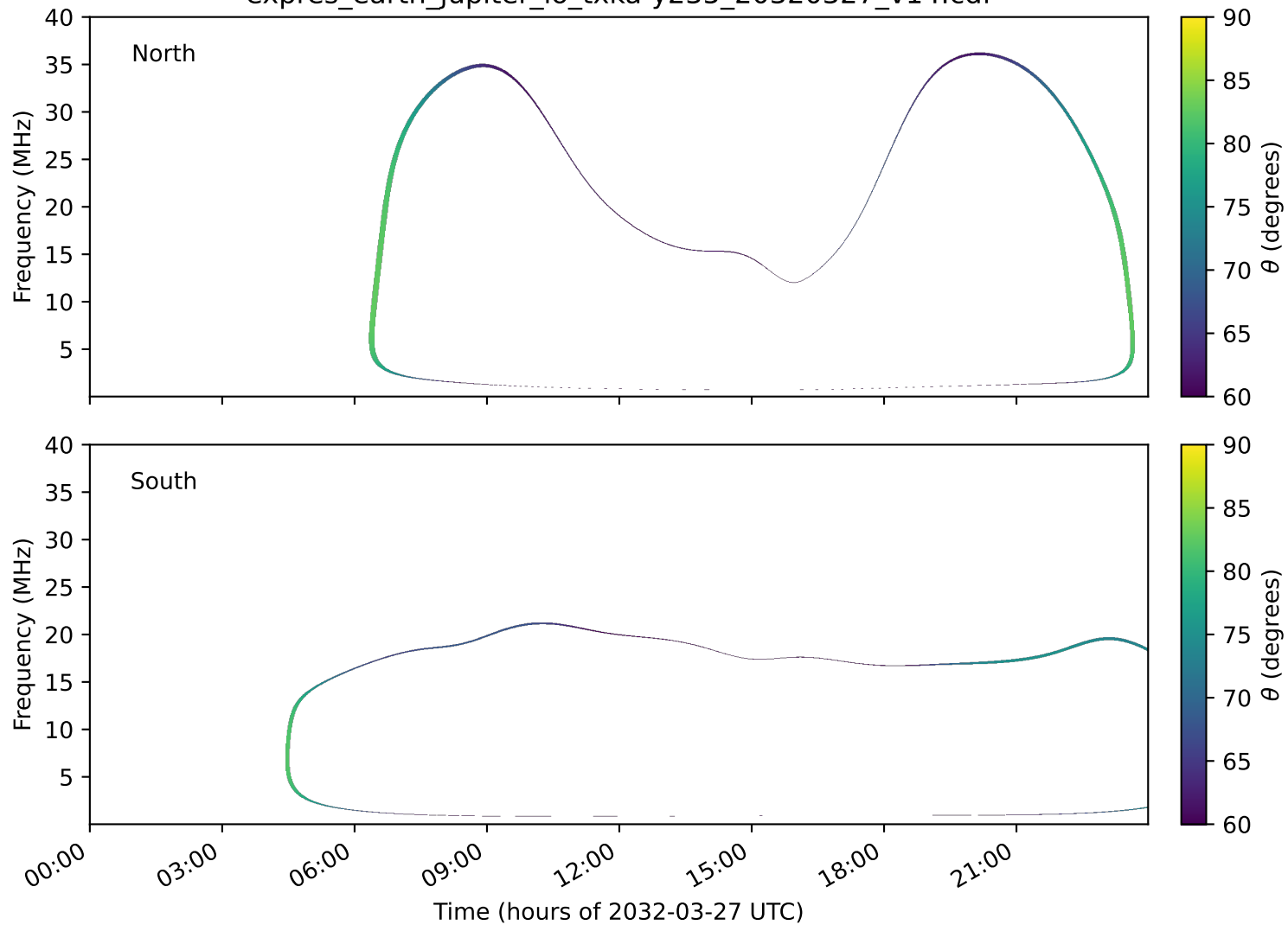
expres_earth_jupiter_io_txka-y235_20320327_v14.cdf
