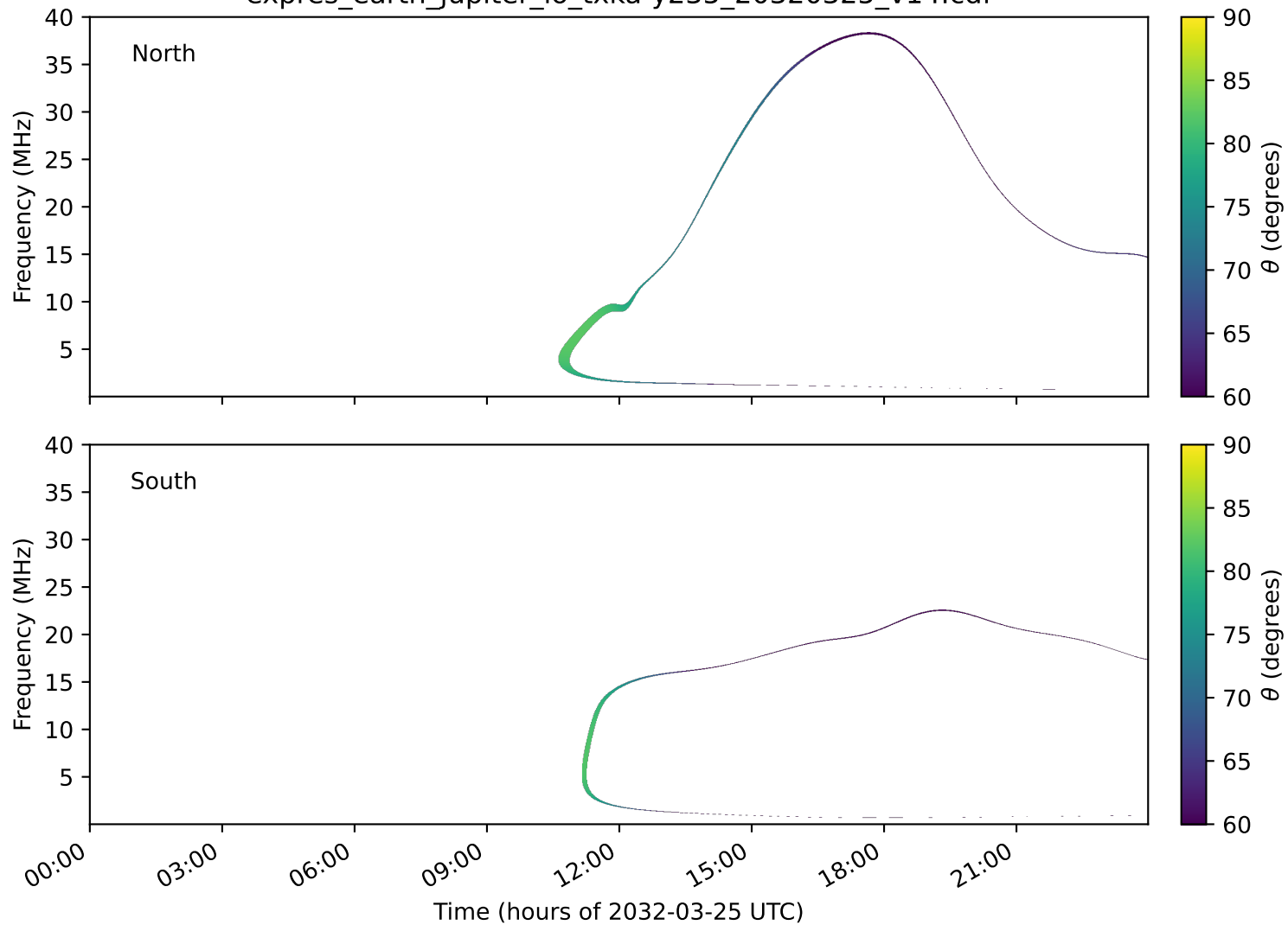
expres_earth_jupiter_io_txka-y235_20320325_v14.cdf
