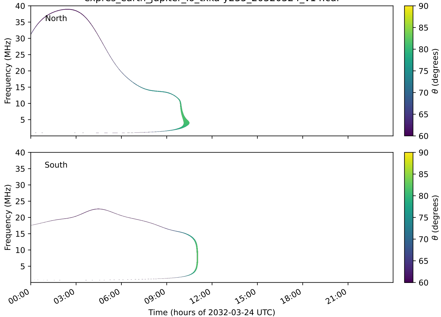
expres_earth_jupiter_io_txka-y235_20320324_v14.cdf
