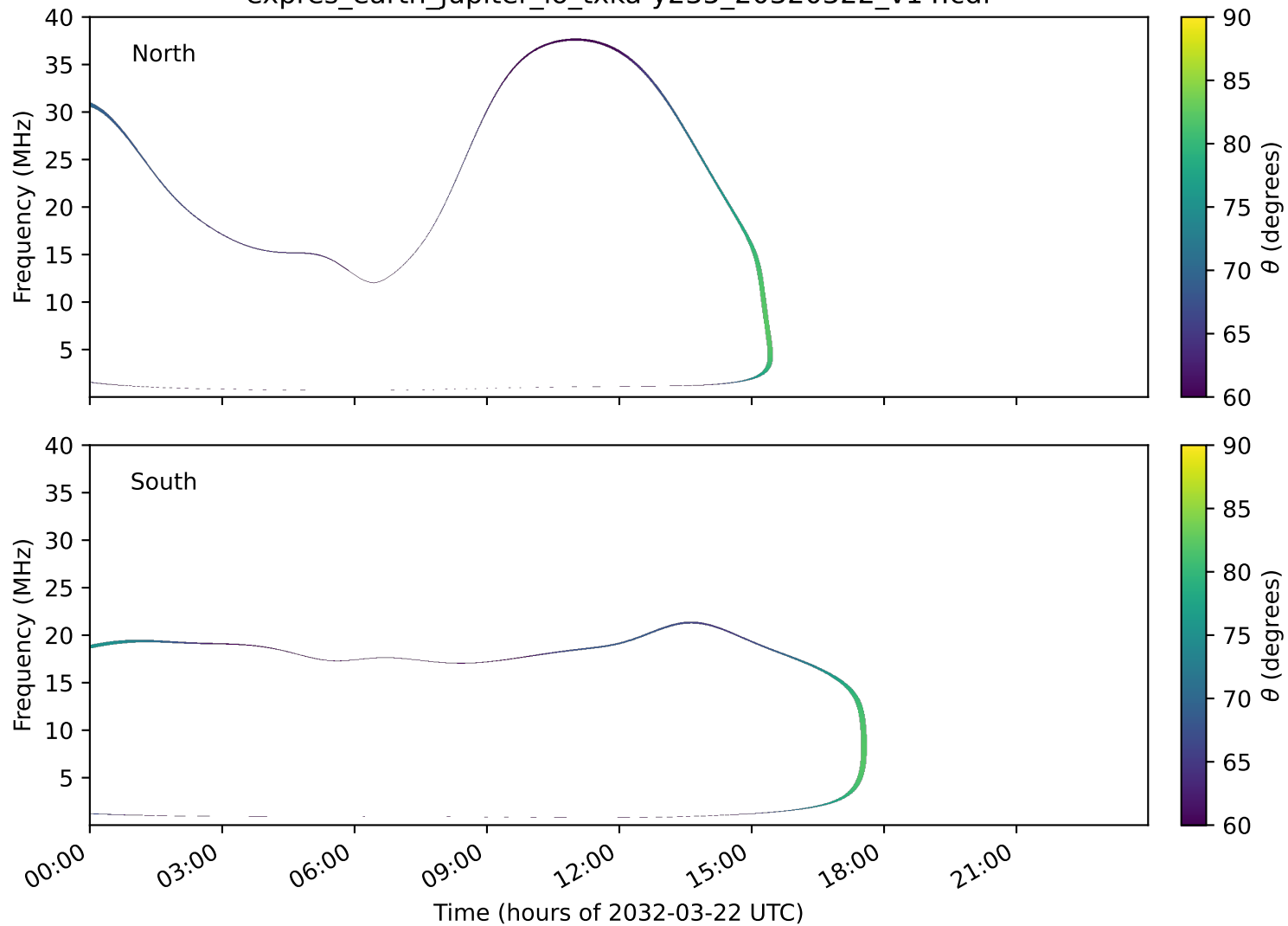
expres_earth_jupiter_io_txka-y235_20320322_v14.cdf
