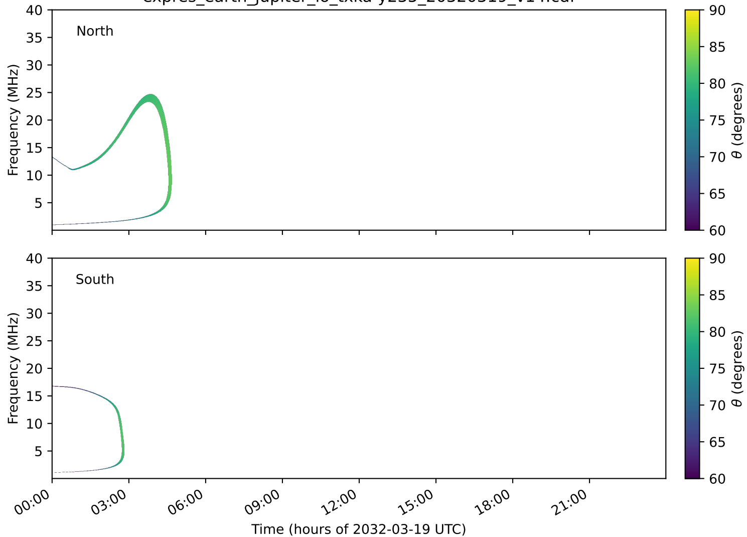
expres_earth_jupiter_io_txka-y235_20320319_v14.cdf
