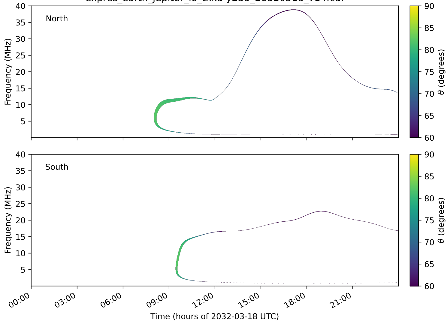
expres_earth_jupiter_io_txka-y235_20320318_v14.cdf
