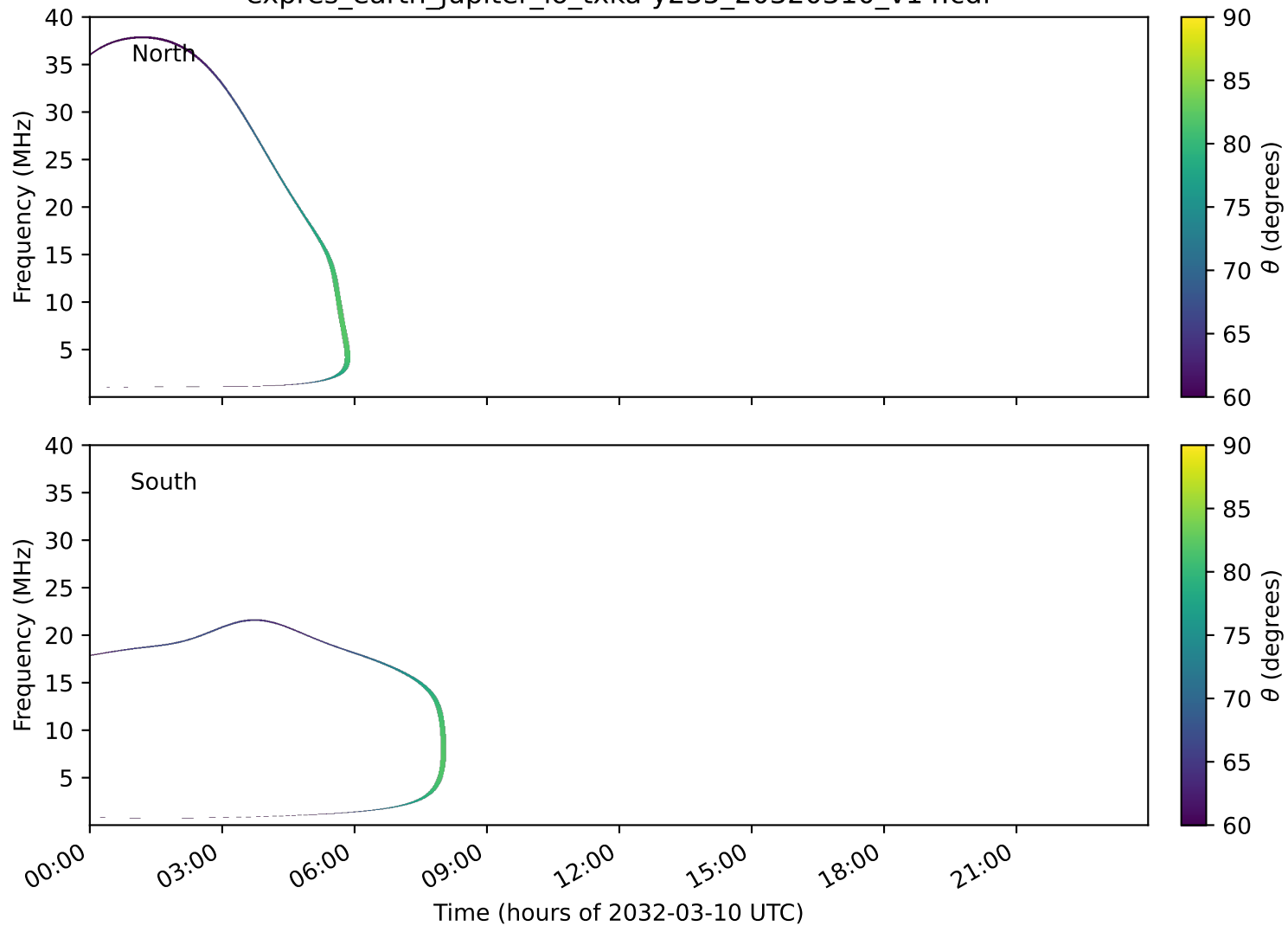
expres_earth_jupiter_io_txka-y235_20320310_v14.cdf
