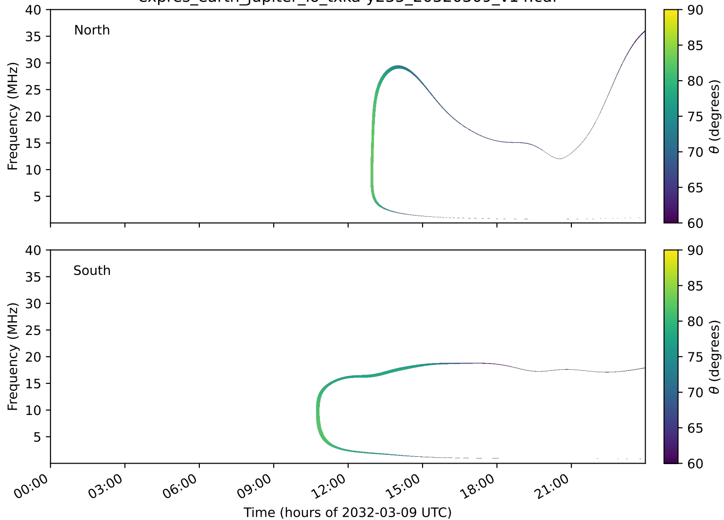
expres_earth_jupiter_io_txka-y235_20320309_v14.cdf
