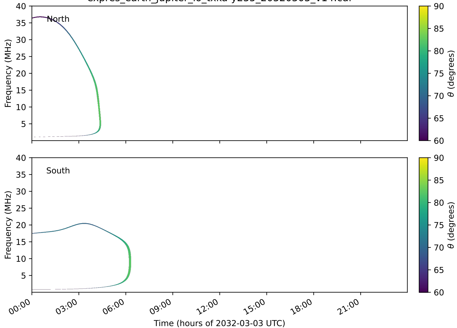
expres_earth_jupiter_io_txka-y235_20320303_v14.cdf
