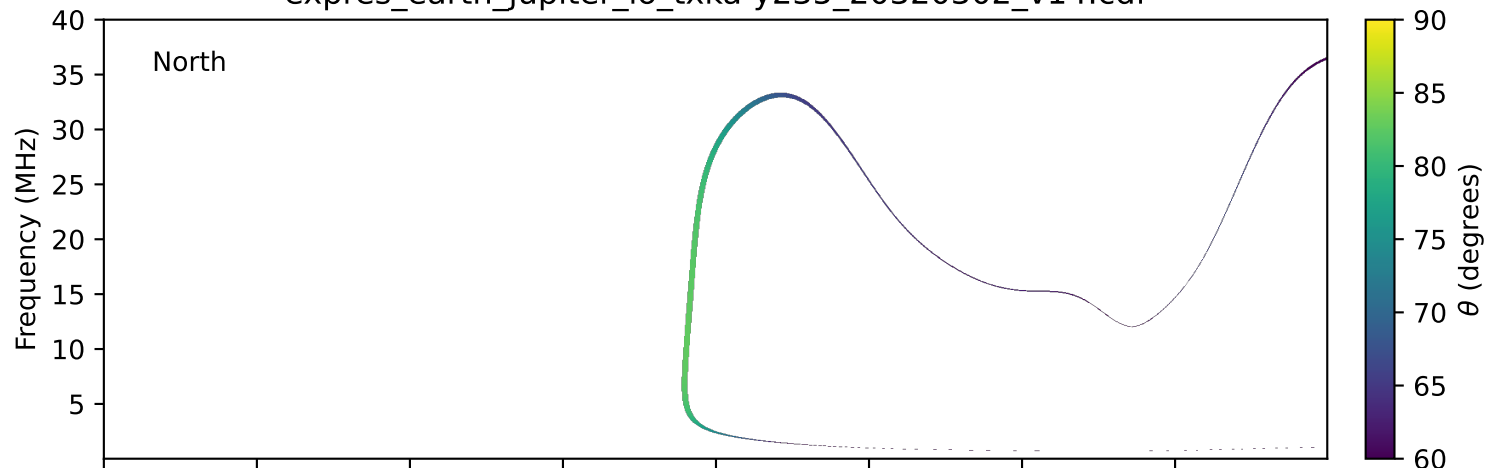
expres_earth_jupiter_io_txka-y235_20320302_v14.cdf
