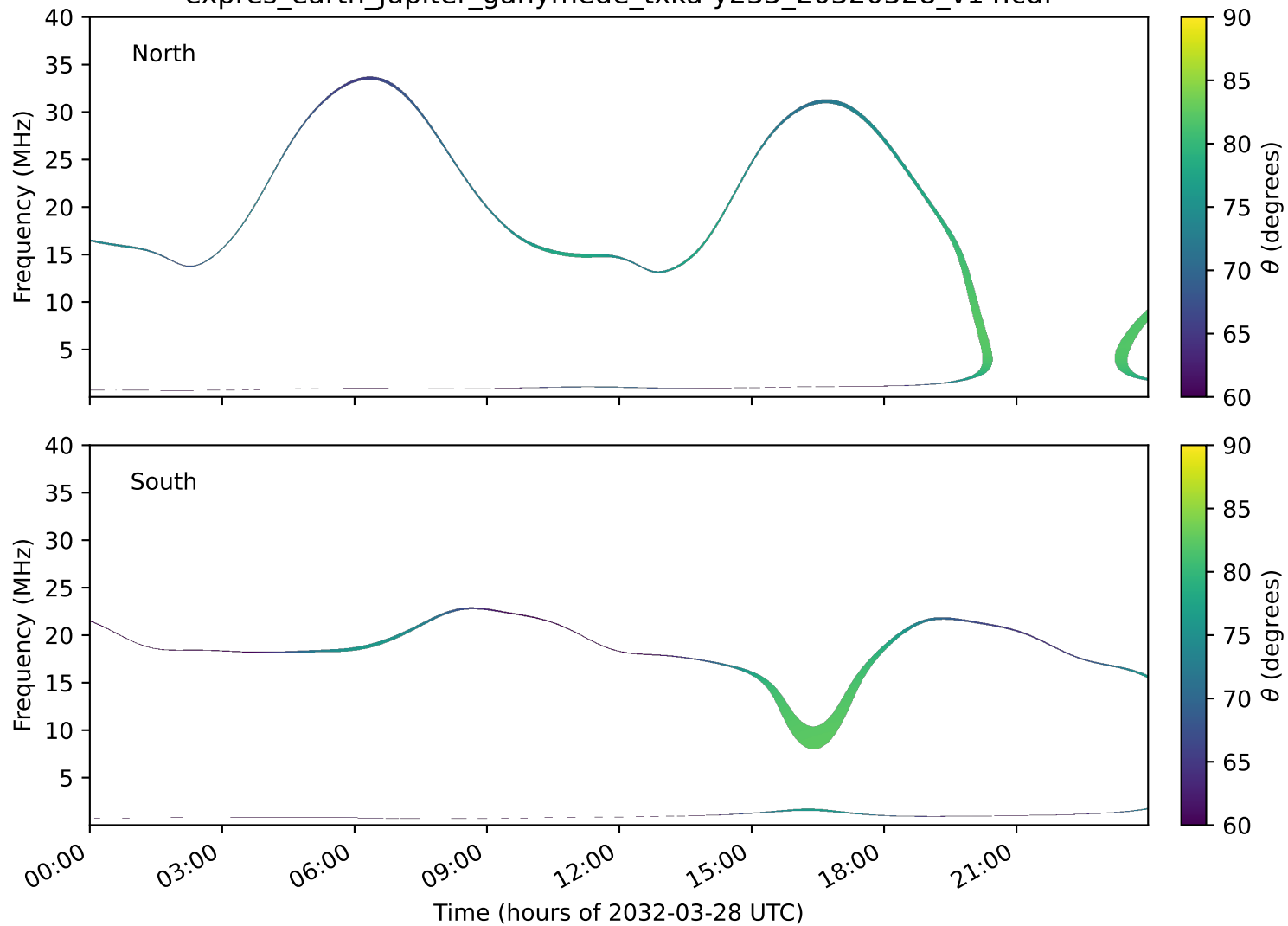
expres_earth_jupiter_ganymede_txka-y235_20320328_v14.cdf
