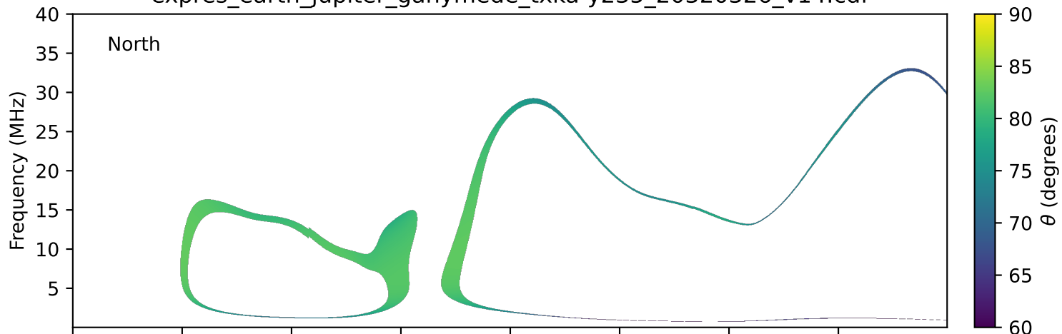
expres_earth_jupiter_ganymede_txka-y235_20320326_v14.cdf
