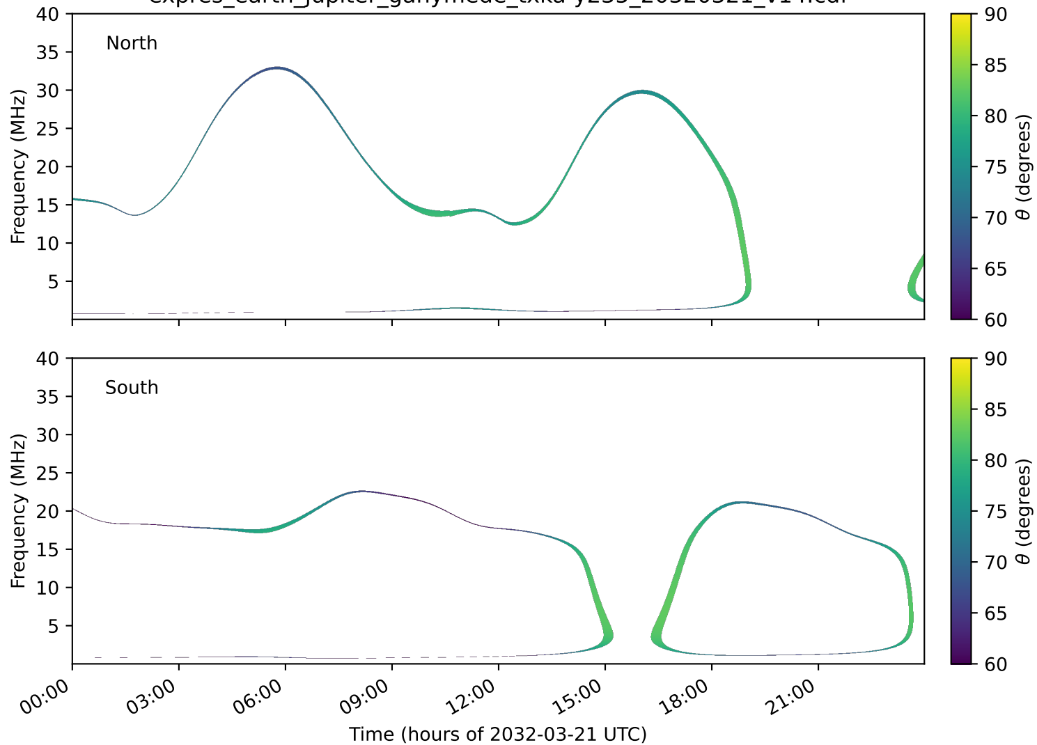
expres_earth_jupiter_ganymede_txka-y235_20320321_v14.cdf
