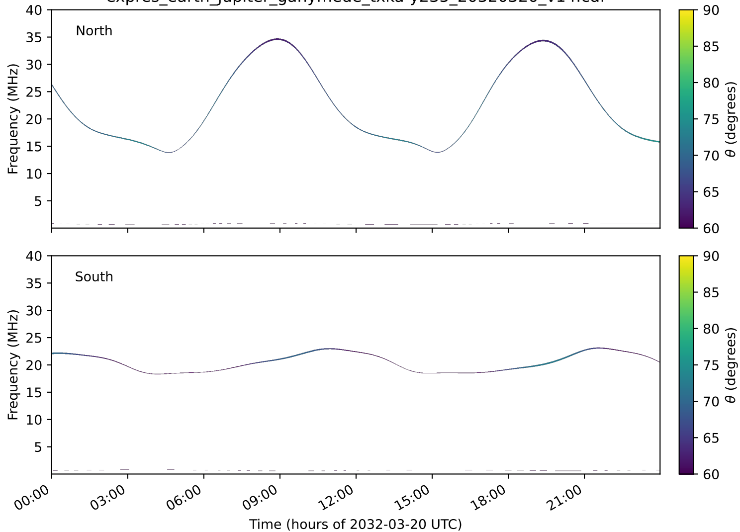
expres_earth_jupiter_ganymede_txka-y235_20320320_v14.cdf
