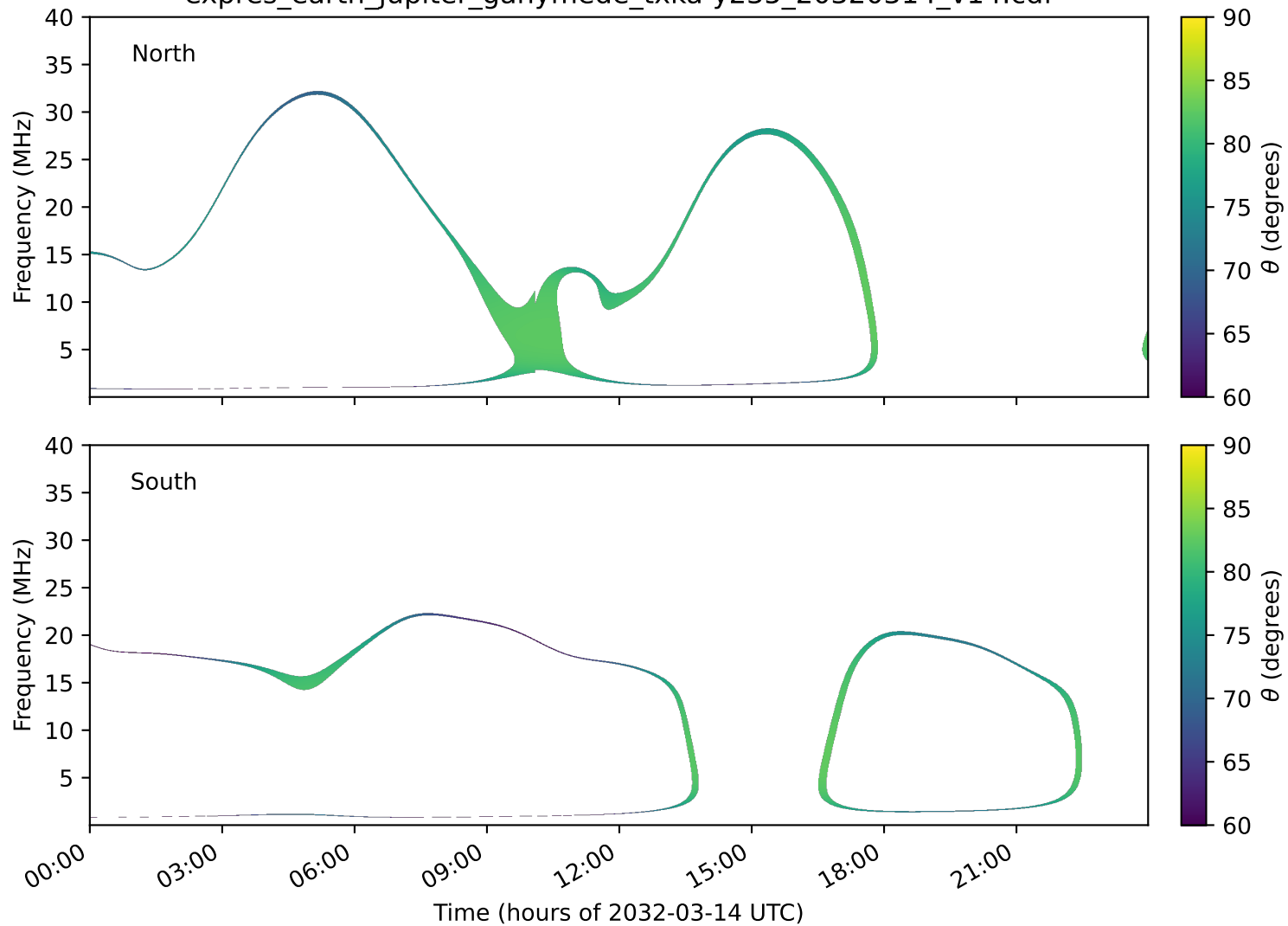
expres_earth_jupiter_ganymede_txka-y235_20320314_v14.cdf
