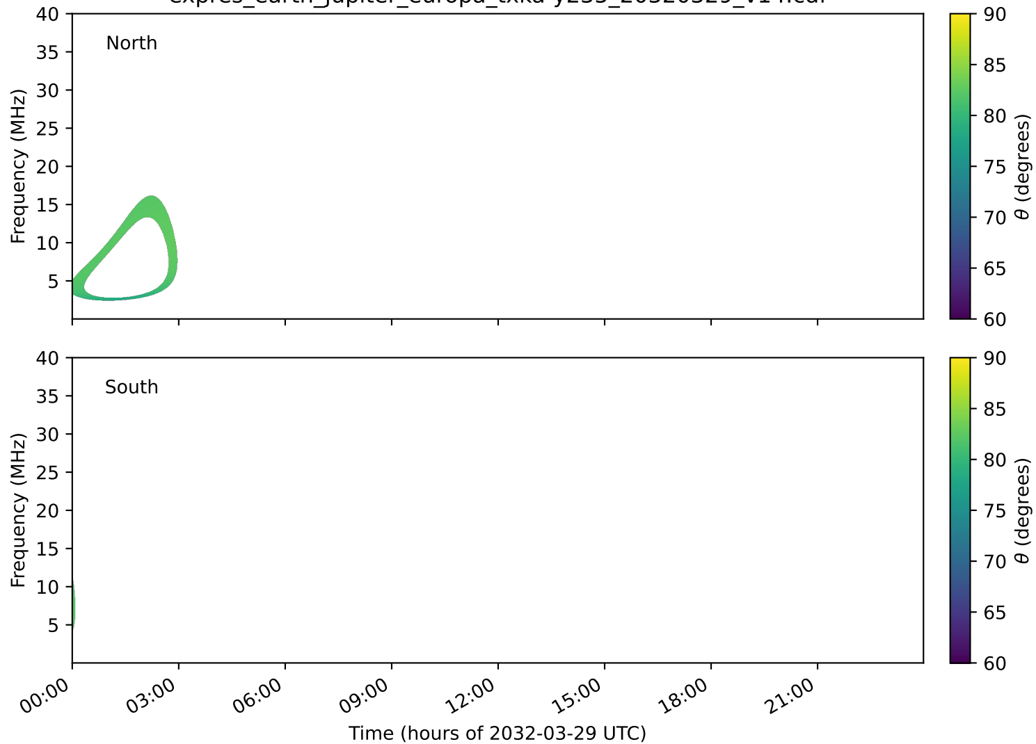
expres_earth_jupiter_europa_txka-y235_20320329_v14.cdf
