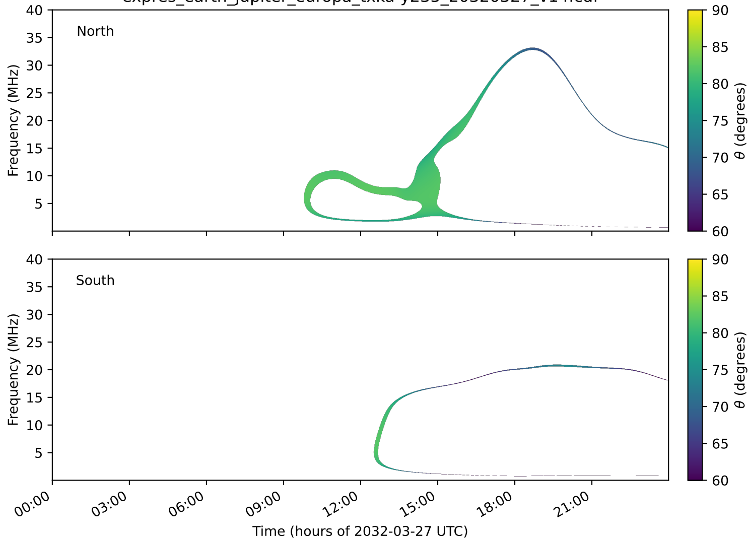
expres_earth_jupiter_europa_txka-y235_20320327_v14.cdf
