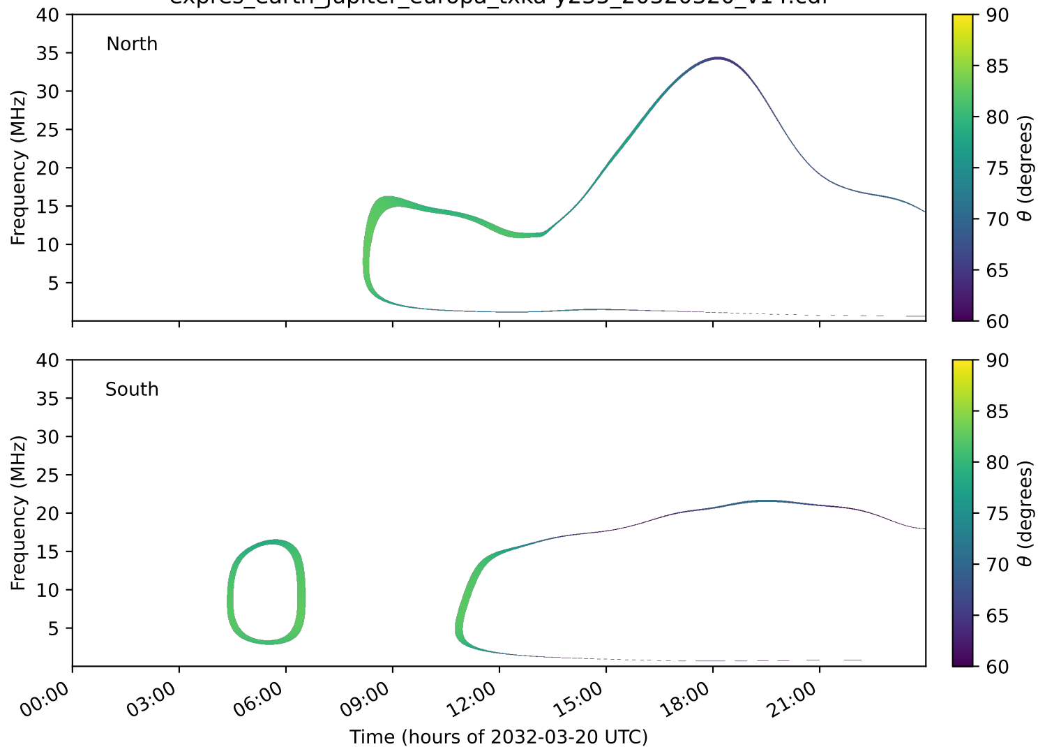
expres_earth_jupiter_europa_txka-y235_20320320_v14.cdf
