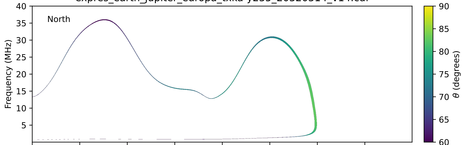
expres_earth_jupiter_europa_txka-y235_20320314_v14.cdf
