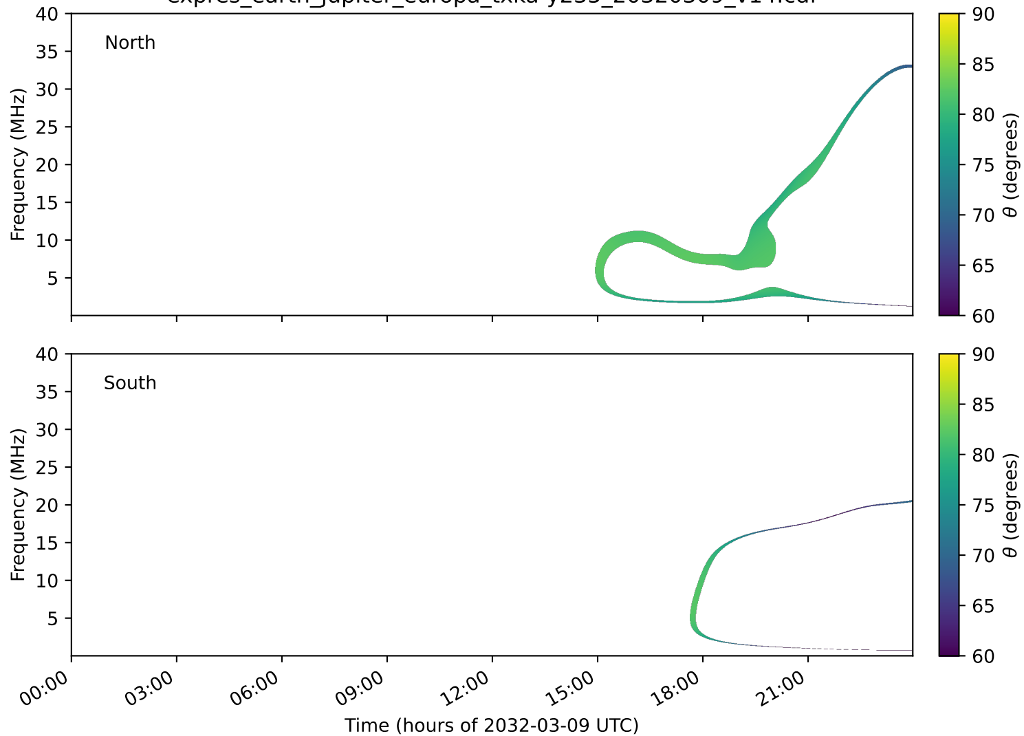
expres_earth_jupiter_europa_txka-y235_20320309_v14.cdf
