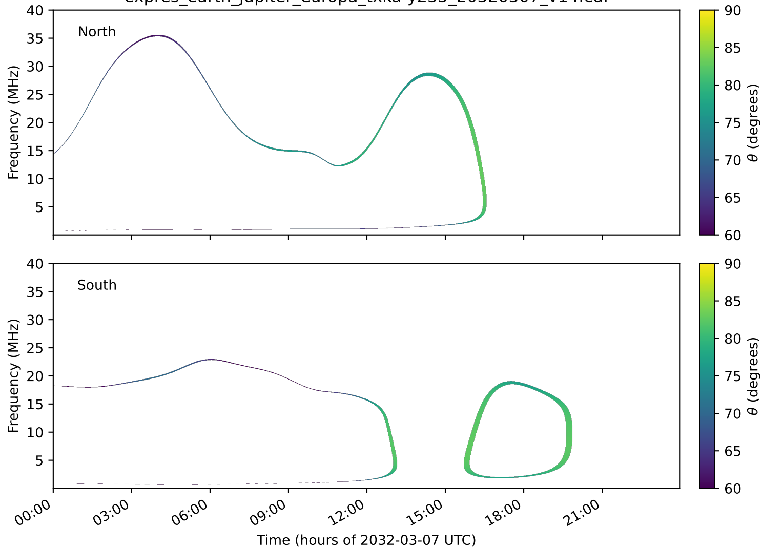
expres_earth_jupiter_europa_txka-y235_20320307_v14.cdf
