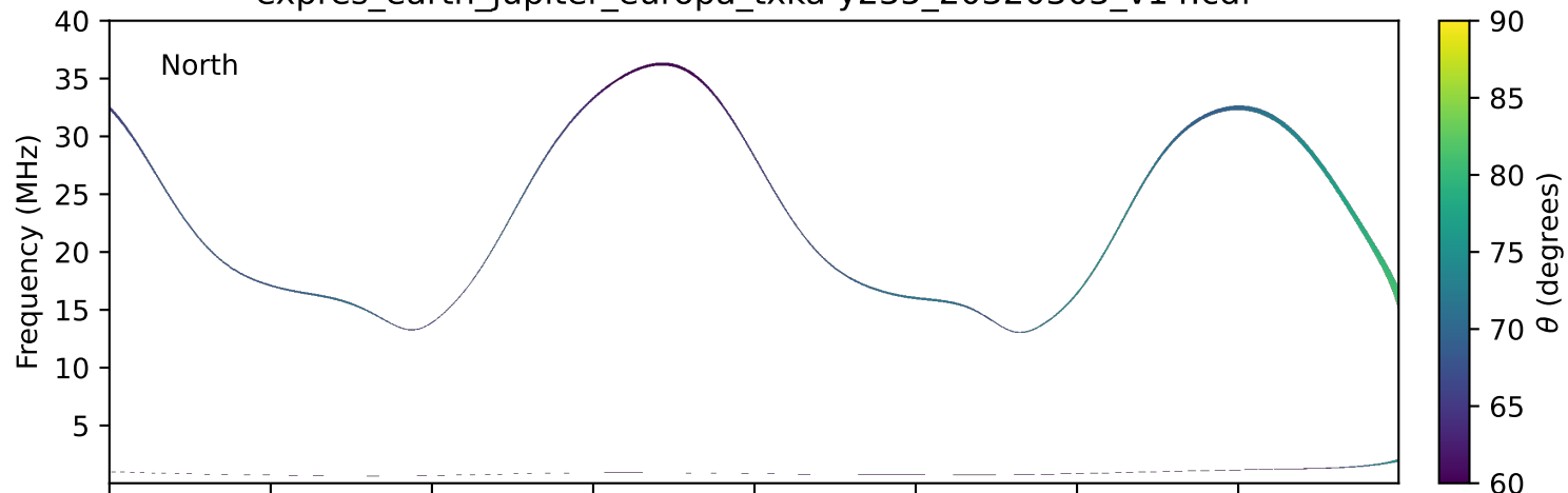
expres_earth_jupiter_europa_txka-y235_20320303_v14.cdf
