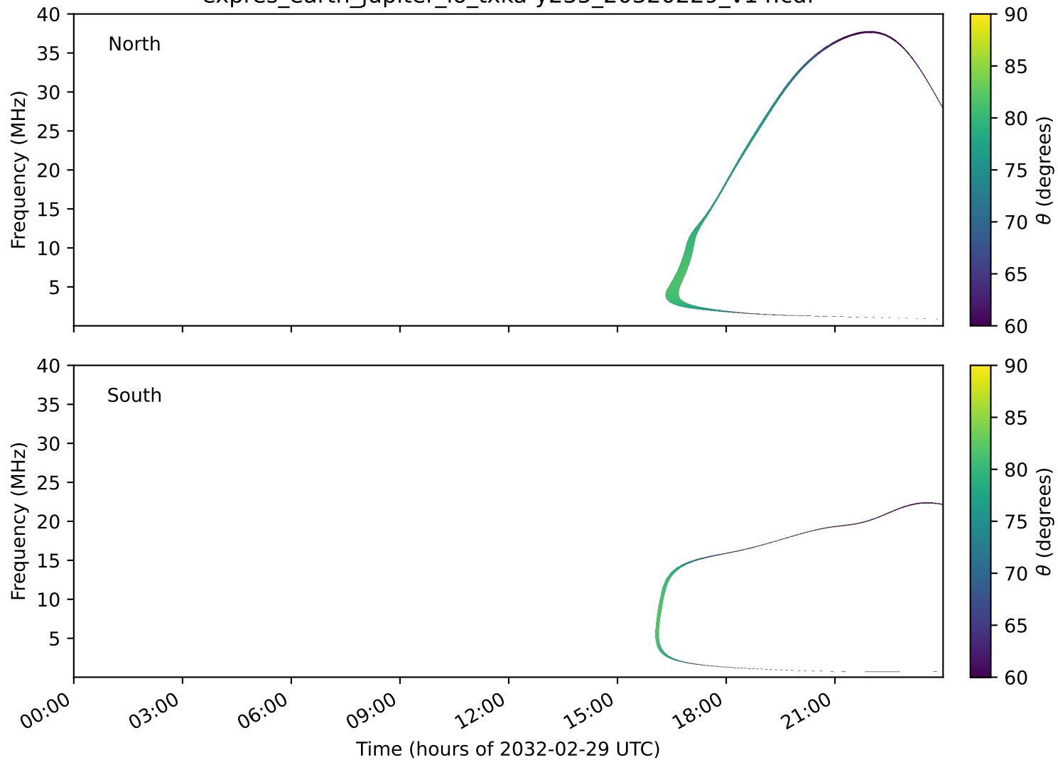
expres_earth_jupiter_io_txka-y235_20320229_v14.cdf
