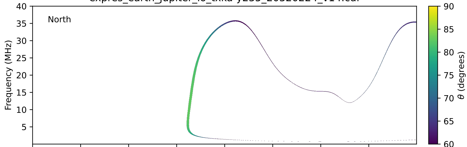
expres_earth_jupiter_io_txka-y235_20320224_v14.cdf
