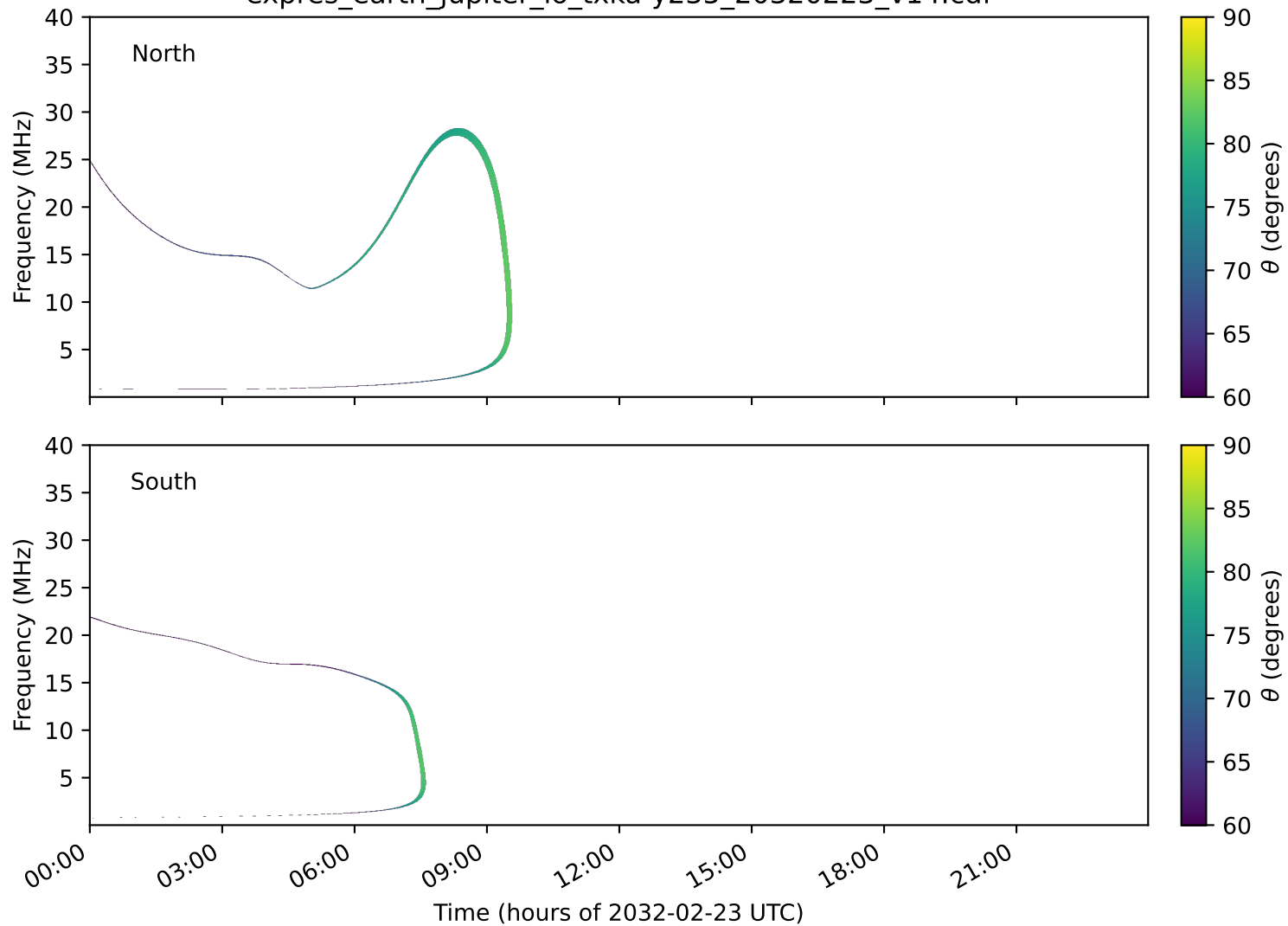
expres_earth_jupiter_io_txka-y235_20320223_v14.cdf
