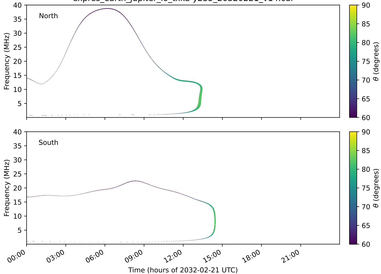
expres_earth_jupiter_io_txka-y235_20320221_v14.cdf
