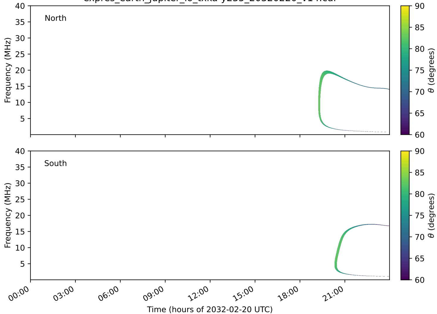
expres_earth_jupiter_io_txka-y235_20320220_v14.cdf
