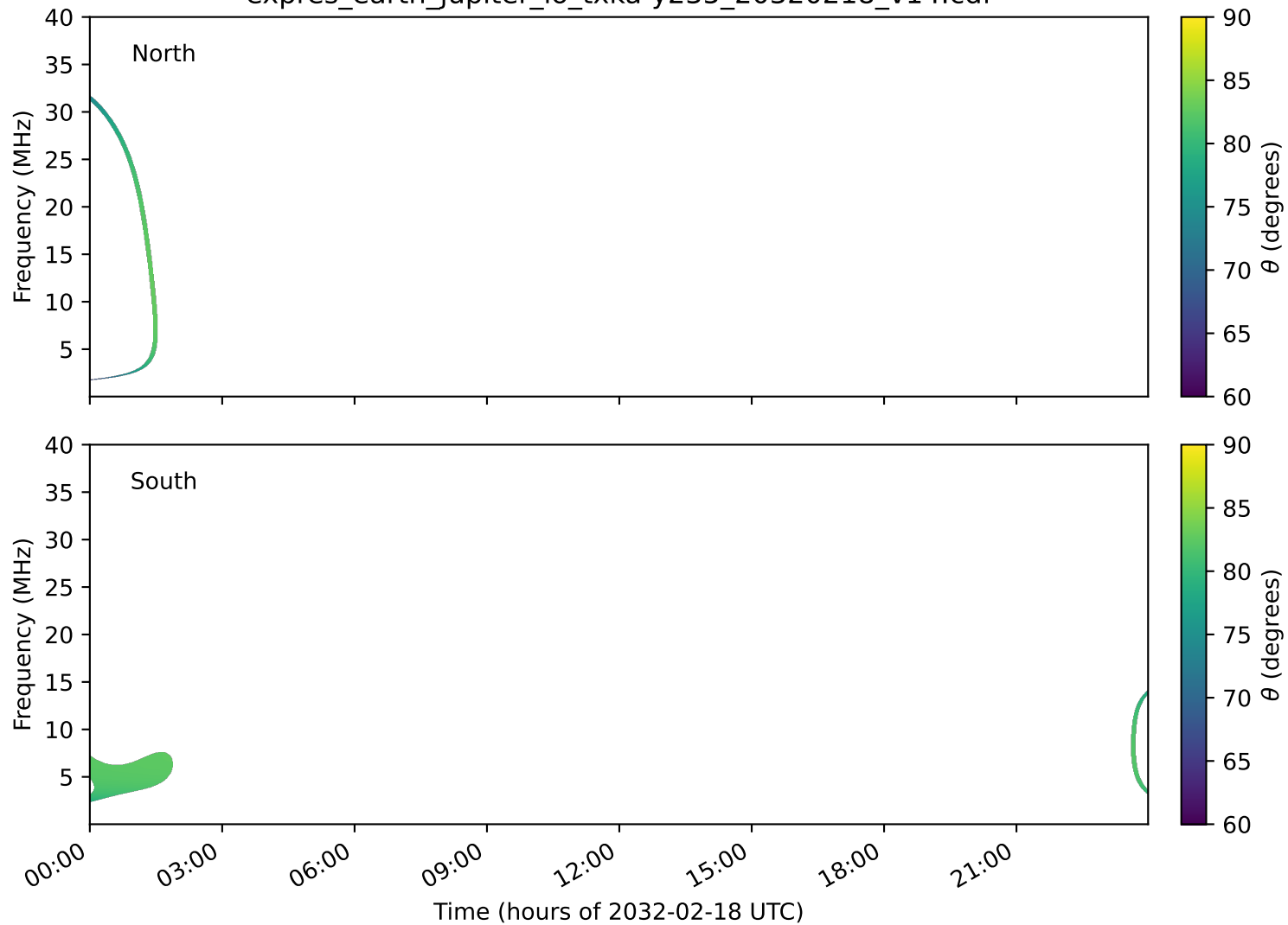
expres_earth_jupiter_io_txka-y235_20320218_v14.cdf
