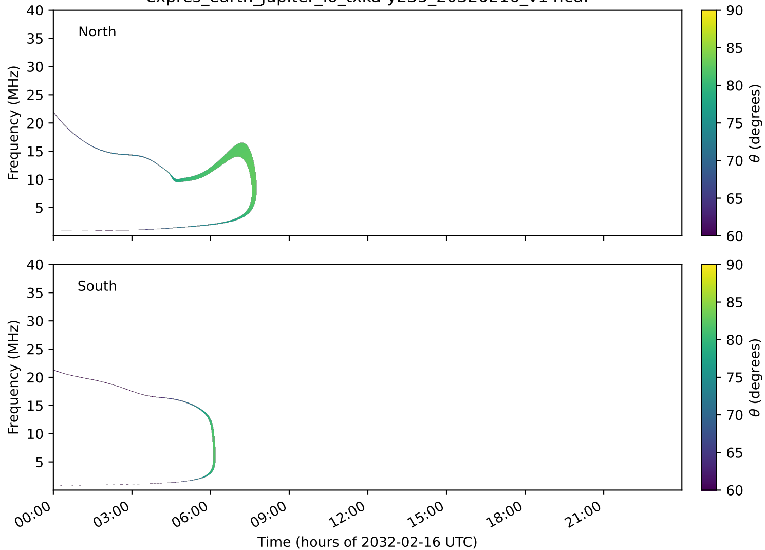
expres_earth_jupiter_io_txka-y235_20320216_v14.cdf
