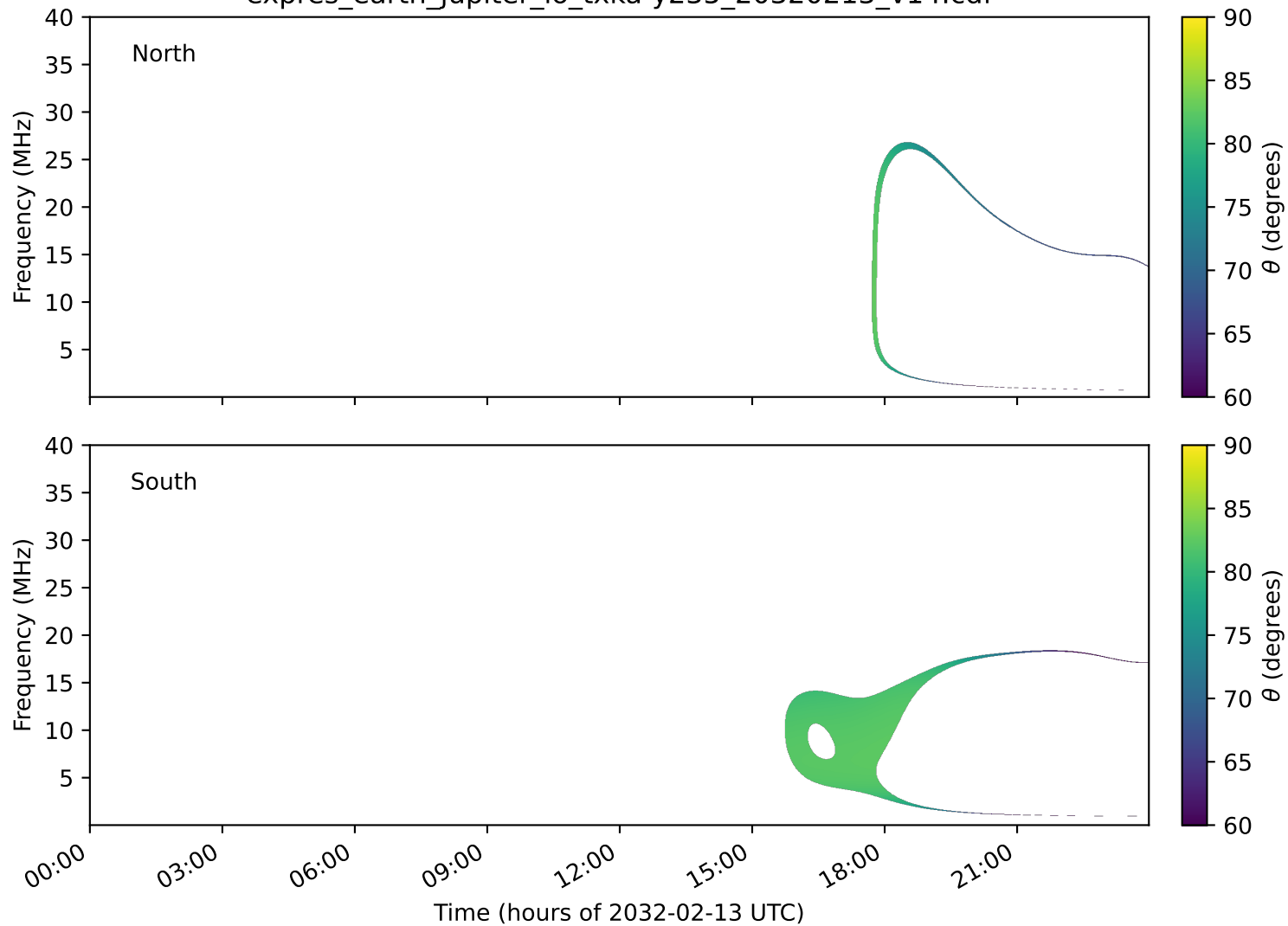
expres_earth_jupiter_io_txka-y235_20320213_v14.cdf
