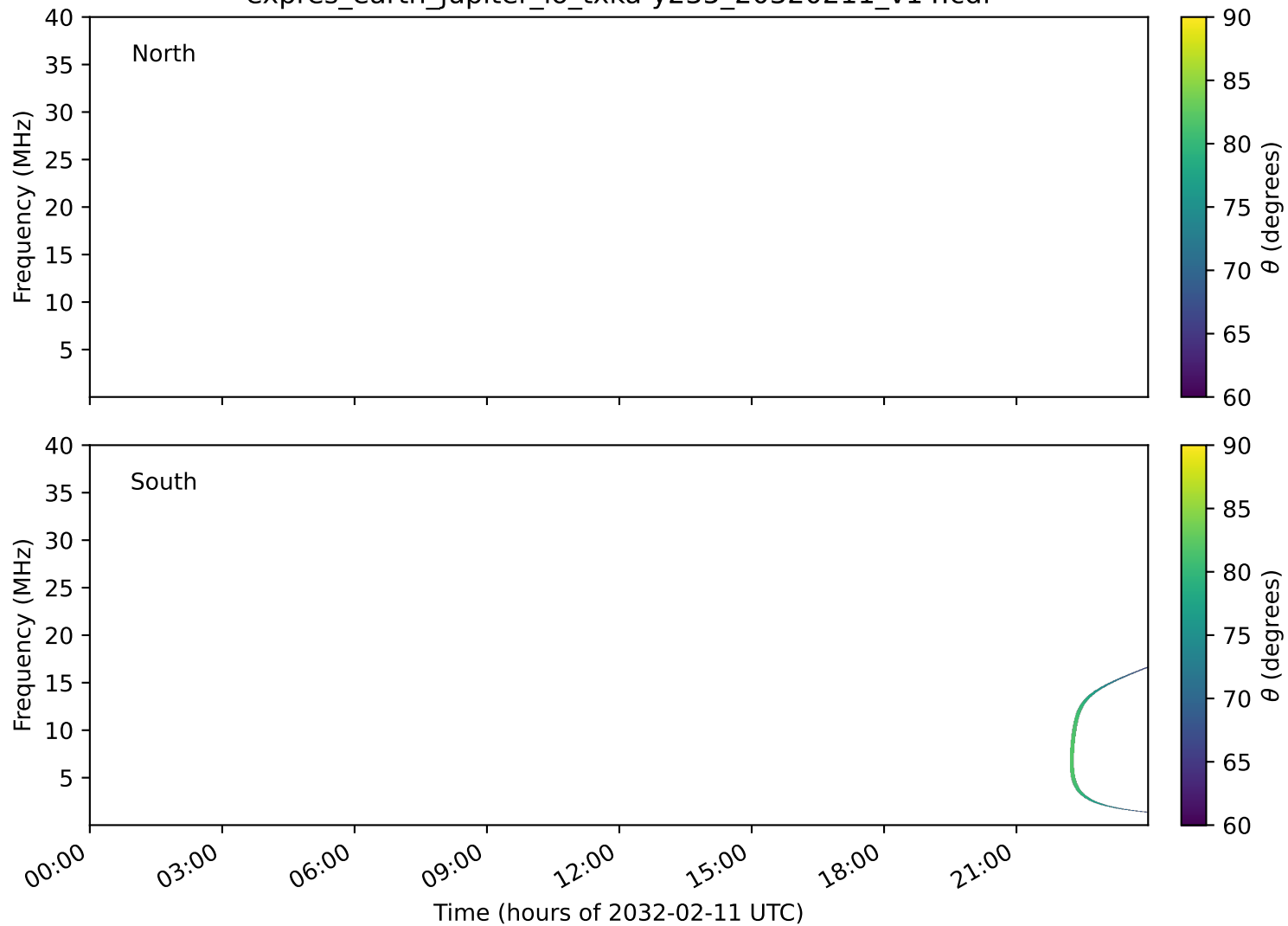
expres_earth_jupiter_io_txka-y235_20320211_v14.cdf
