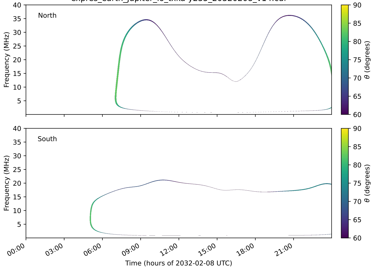
expres_earth_jupiter_io_txka-y235_20320208_v14.cdf
