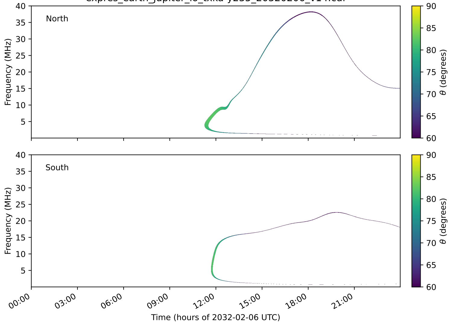
expres_earth_jupiter_io_txka-y235_20320206_v14.cdf
